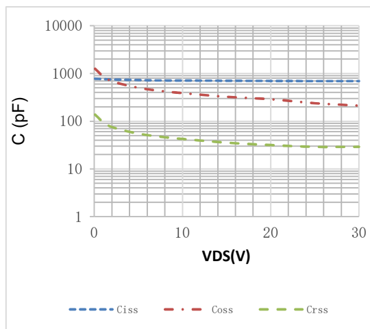
Fig.2 Capacitance Characteristics
